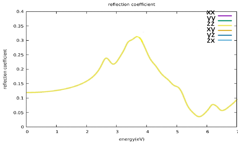
Figure 8: Reflectivity R(\omega) .
