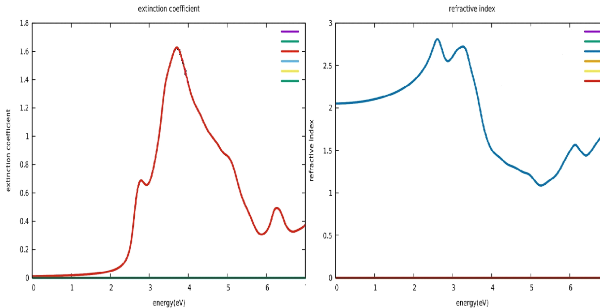
Figure7: (a) Extinction coefficient k(\omega) and (b) Refractive index n(\omega) .
