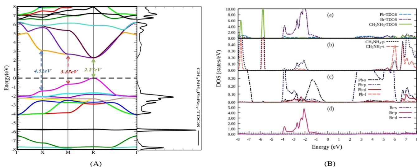
Figure 3: (A) Band structure and (B) Partial density of state for \text{CH}_3\text{NH}_3\text{PbBr}_3 , where zero energy corresponds to the Fermi level [19].
