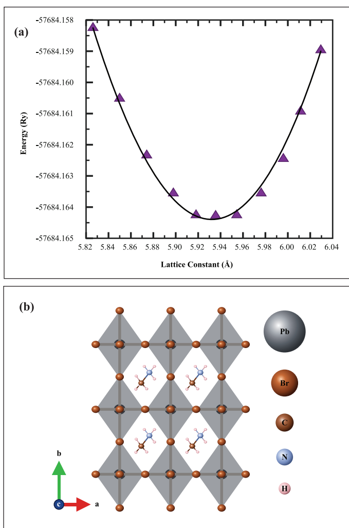
Figure 1: (a) Calculated total energy vs lattice constant cubic CH_3NH_3PbBr_3 using WC-GGA potential. (b) The schematic optimized structure of CH_3NH_3PbBr_3 perovskites.
