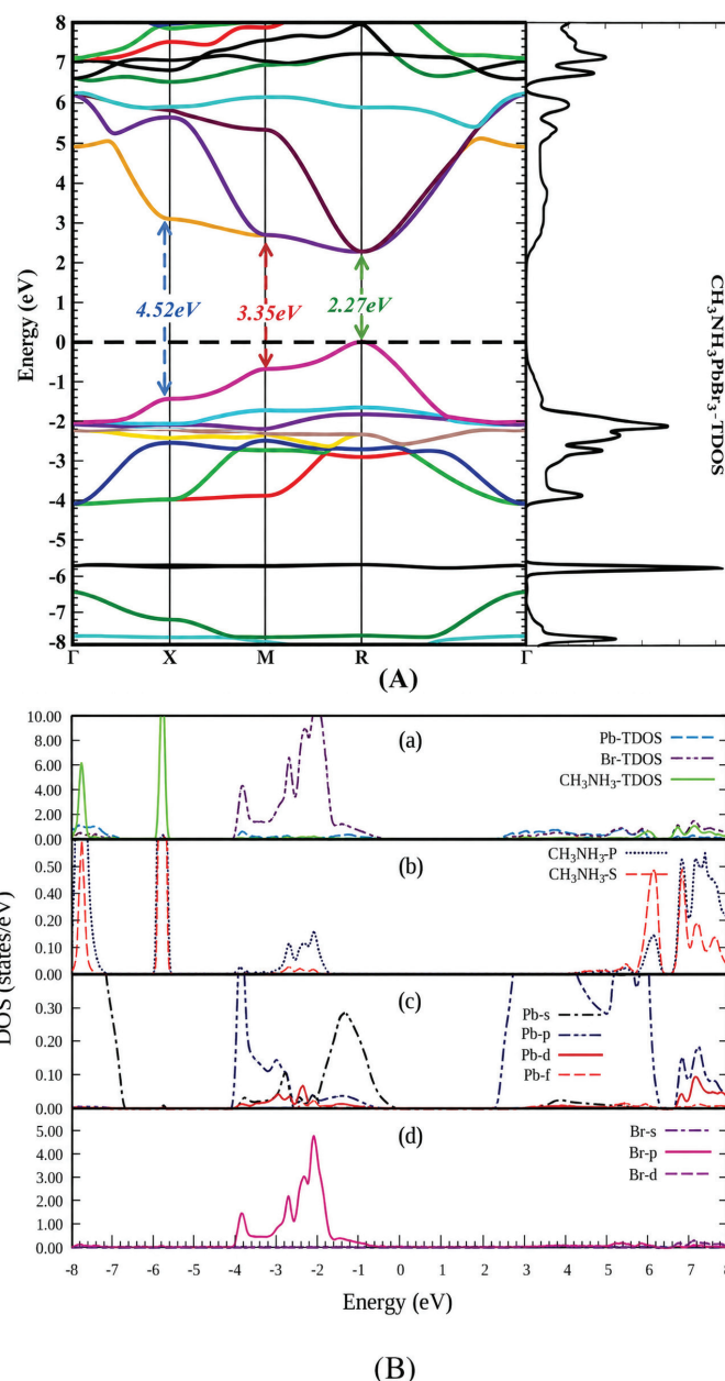
Figure 3: (A) Band structure and (B) Partial density of state for \text{CH}_3\text{NH}_3\text{PbBr}_3 , where zero energy corresponds to the Fermi level.
