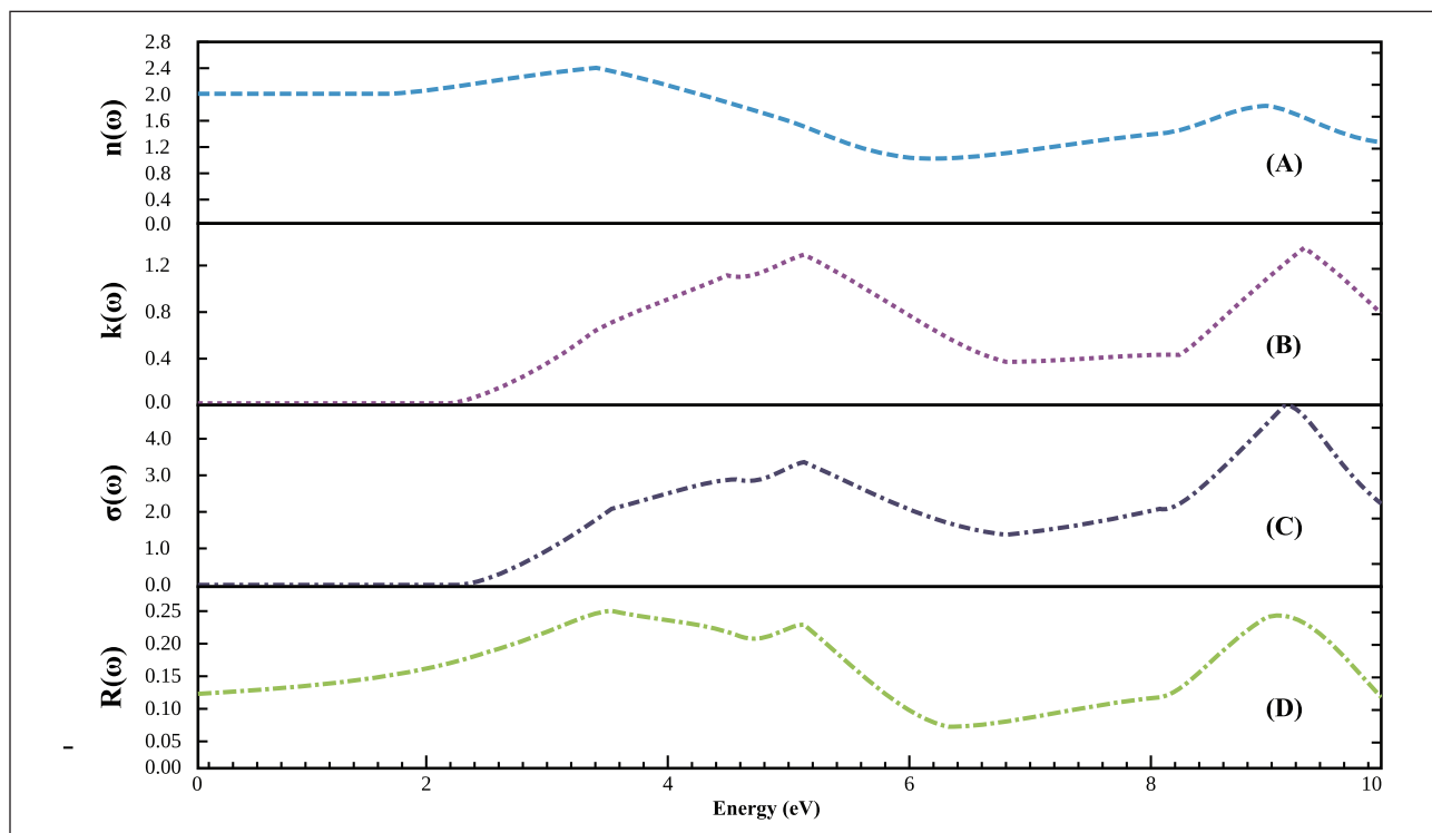
Figure 10: Incident photon energy dependence: (A) Refractive index - n(\omega) , (B) Extinction coefficient - k(\omega) , (C) Optical conductivity - \sigma(\omega) , and (D) Reflection coefficient - R(\omega) of \text{CH}_3\text{NH}_3\text{PbBr}_3 .
