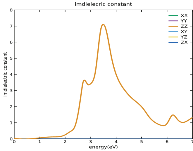
Figure 5: Spectra of optical properties as a function of photon energy for lead free halide double perovskite \text{Cs}_2\text{AgBiBr}_6 , (a) Imaginary part \epsilon_2(\omega) and (b) real part \epsilon_1(\omega) of dielectric function.
