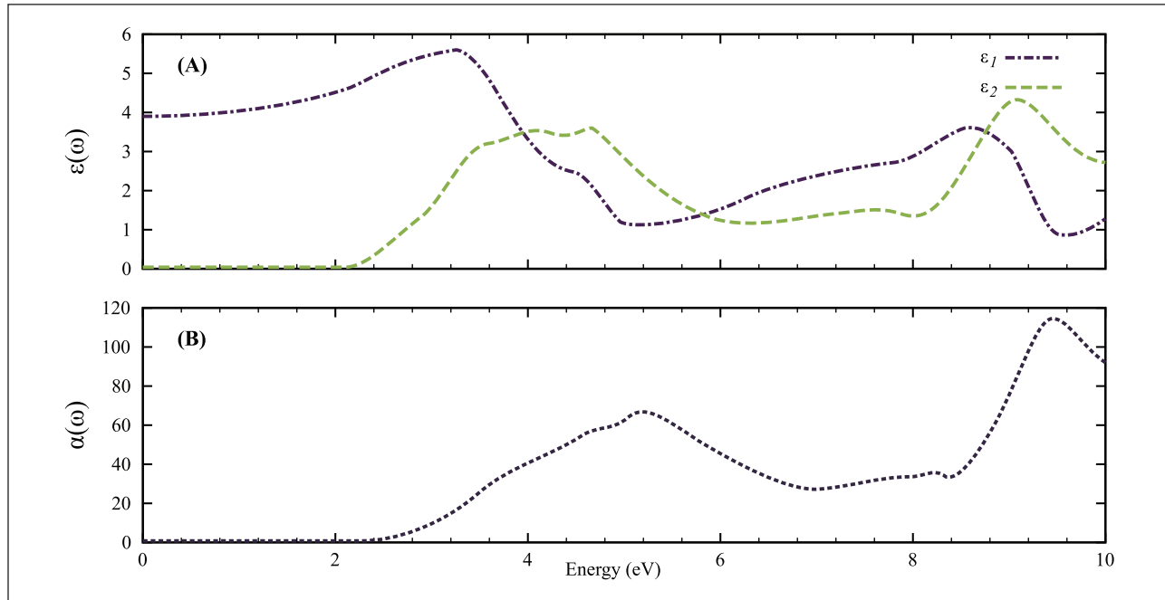
Figure 9: The plotted curve between photon energy in (eV) vs, (A) Dielectric parameters \epsilon_1(\omega) real and \epsilon_2(\omega) imaginary and (B) Absorption coefficient \alpha(\omega) of \text{CH}_3\text{NH}_3\text{PbBr}_3 .
