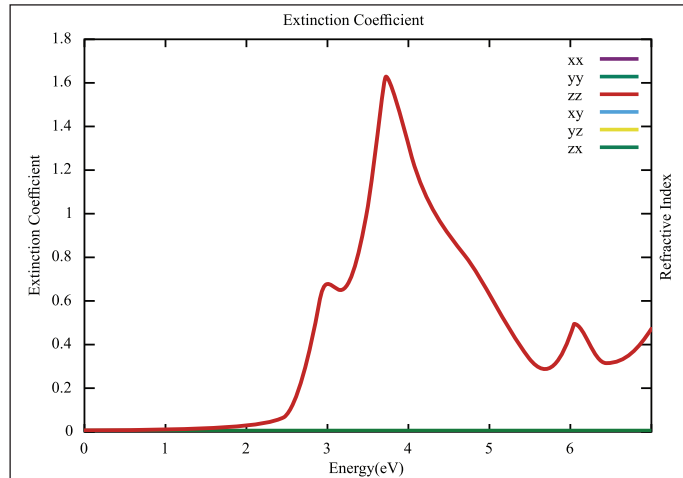
Figure7: (a) Extinction coefficient k(\omega) and (b) Refractive index n(\omega) .
